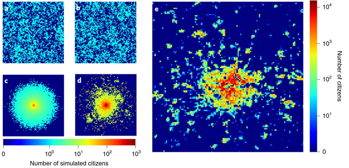
Fig. 49. Morphologies retrieved from different models compared with London: (a) Lévy flights, (b) gravity model, (c) Individual Mobility Model, (d) Collective Mobility Model, (e) London. Simulations were run until population distributions converged. Source: From [170].
