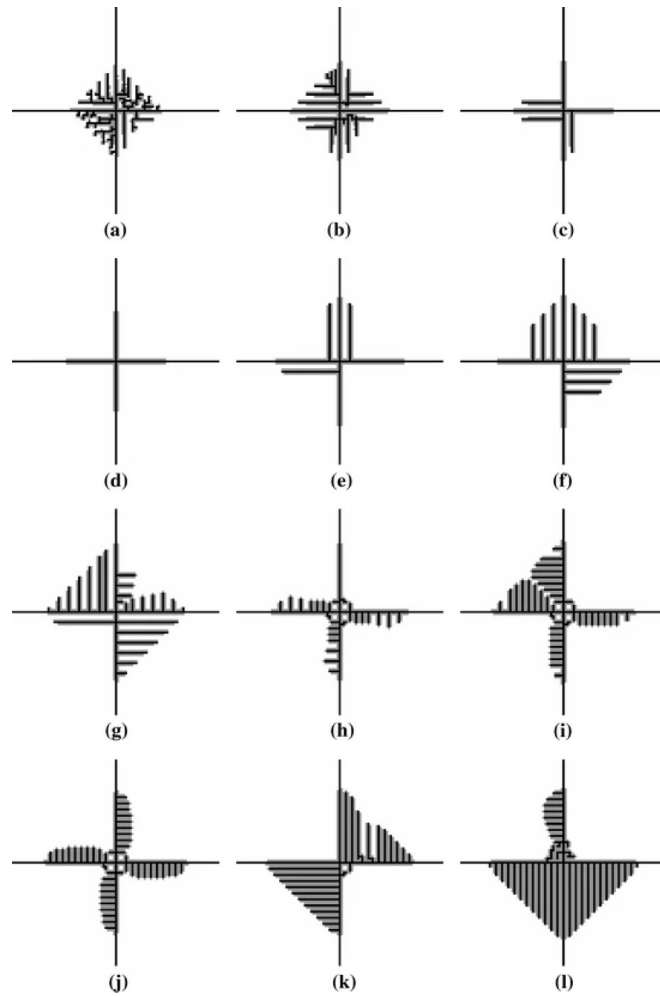
Fig. 33. Long-run equilibrium morphologies as \gamma varies for fixed \beta = 0.25 . (a) \gamma = 0.00 , (b) 0.09, (c) 0.11, ..., (l) 0.45. Increasing \gamma suppresses dendritic growth and induces linear and grid-like morphologies. Source: From [129].
