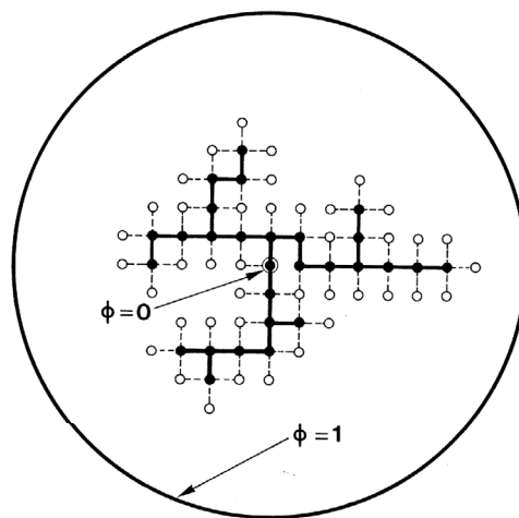
Fig. 39. Stochastic model of electric breakdown on a lattice, proposed in [150]. The central point represents one electrode, while the other is modeled as a distant circular boundary. The discharge pattern is shown by black dots connected with thick lines and is treated as equipotential. Dashed bonds indicate all possible growth directions, with transition probabilities proportional to the local electric field. \phi is the electric potential: the discharge pattern is equipotential ( \phi = 0 ) – the other boundary condition imposes \phi = 1 beyond the external circle. Source: From [150].
