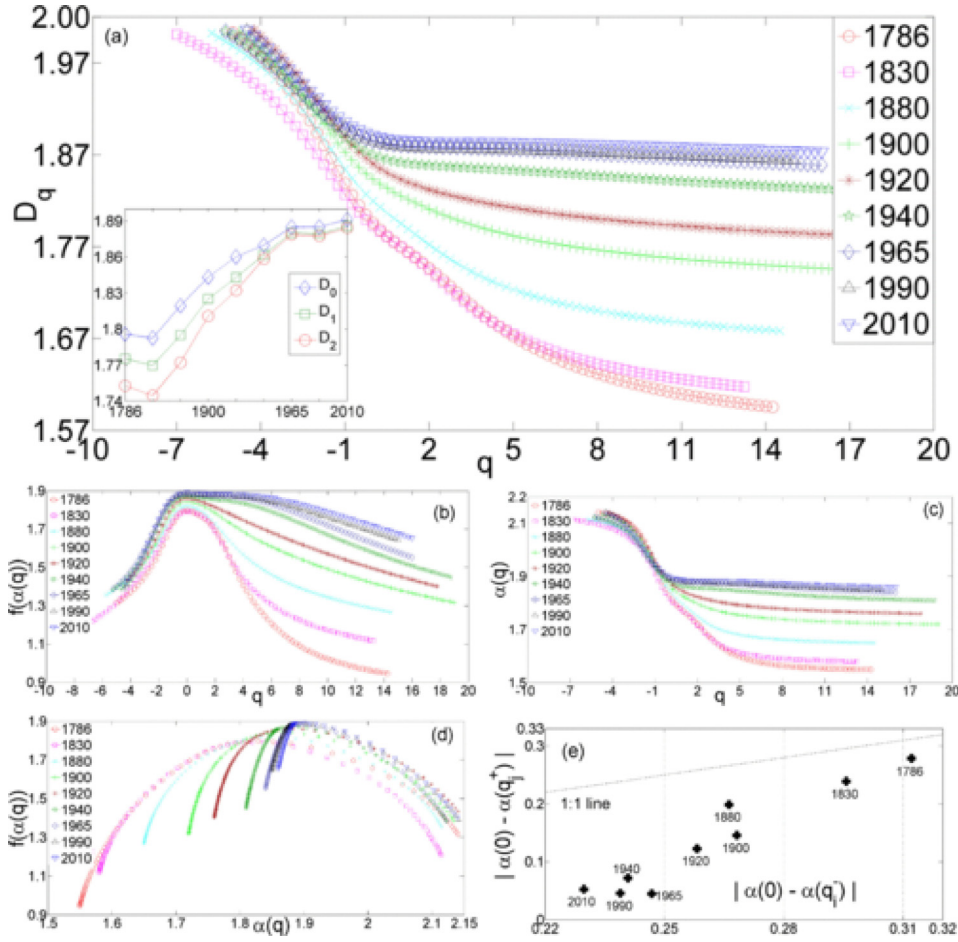
Fig. 9. Multifractal analysis of Greater London's street network intersection point pattern, between 1786 and 2010. (a) Generalized fractal dimensions against q (inset : temporal evolution of D_q for selected values q = 0, 1, 2 ). (b) Fractal dimension of \alpha(q) -sets in function of q . (c) \alpha(q) against q . (d) Multifractal spectrum. (e) Asymmetry of the relative spectrum.
