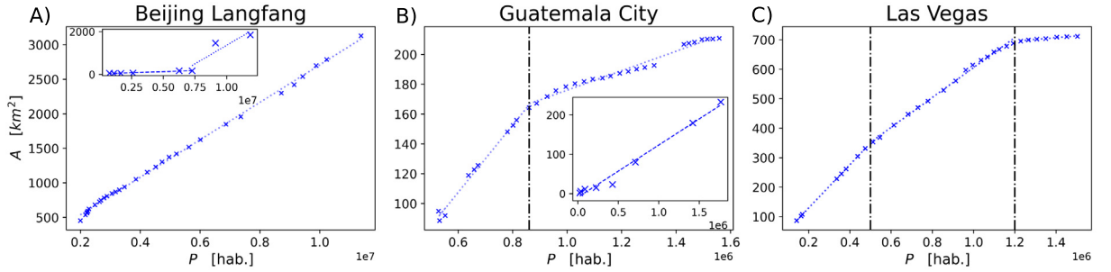
Fig. 21. Illustration of the three growth area against population patterns (A) linear growth (B) piecewise linear growth with density breaking point (C) saturation. The dashed lines mark the breaking points. Insets : area against total population for historical data (from [90]). Source: From [1].
