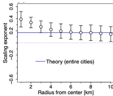
Fig. 18. Scaling exponent \beta for the relation between average building height, \bar{h} , and city population size P , plotted as a function of the radius d from the city center. For the whole city ( d large), the exponent approaches the theoretical prediction \beta = 1/6 [86]. Error bars denote the 95% confidence interval.
