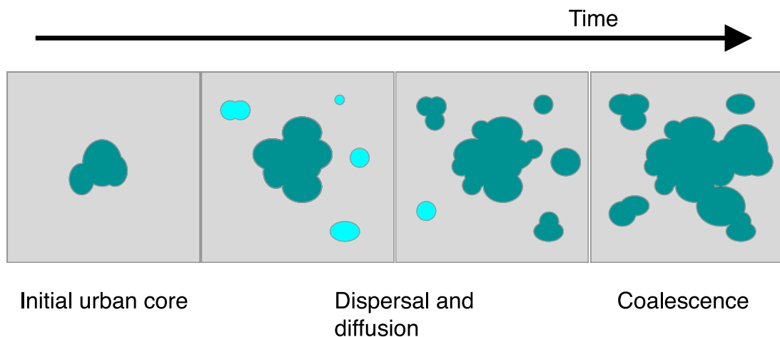
Fig. 2. Typical sequence of urban growth. An initial urban core expands and generates secondary clusters (light blue). Both the core and the peripheral clusters grow through a diffusion-like process and may eventually coalesce.
