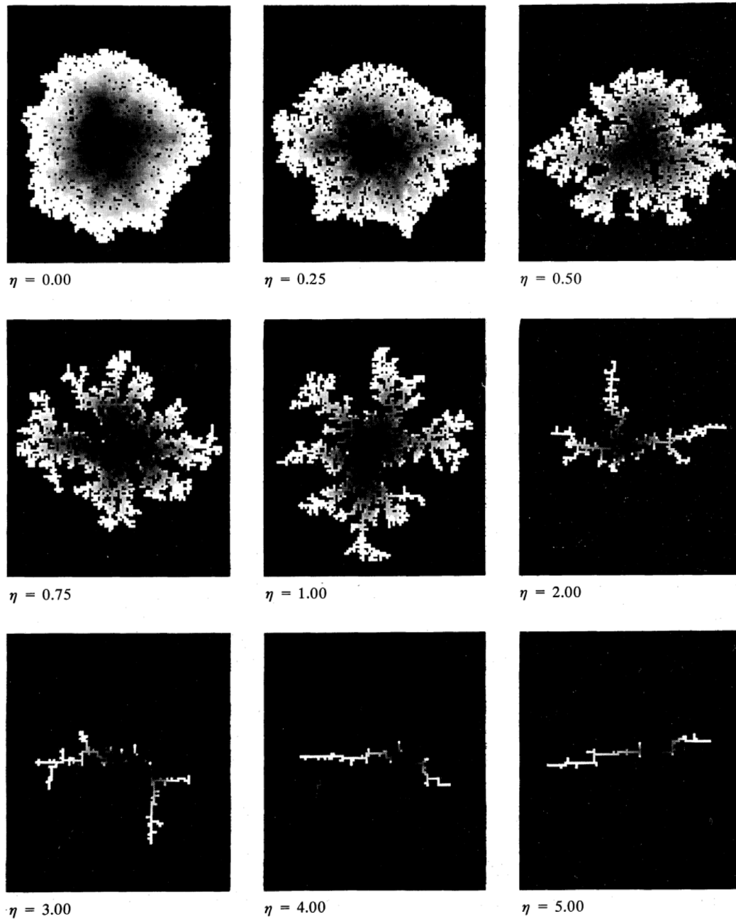
Fig. 40. Simulations of the city shape for increasing values of the ‘planning constraint’ \eta . Source: From [151].
