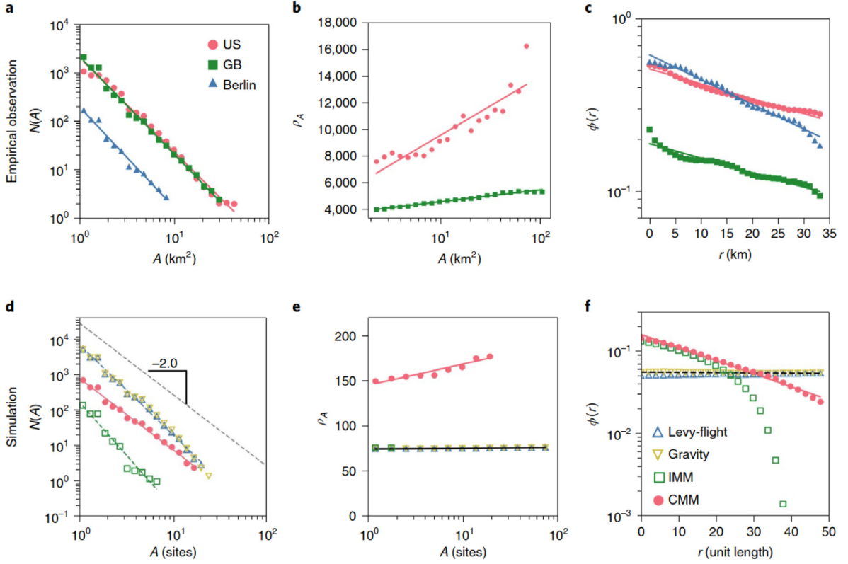
Fig. 50. Comparison between empirical morphology statistics (upper row) and model simulations (lower row). Panels (a) and (d): cluster size statistics; (b) and (e): city density versus size; (c) and (f): radial density profiles. Source: From [170].
