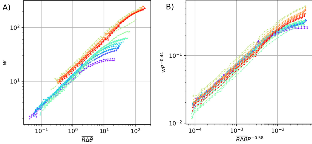
Fig. 23. (A) Roughness of interface against \bar{\ell} = \overline{R\Delta\theta} , for Ningbo, China, for each year between 1985 (purple) and 2015 (red). (B) Rescaled curves according to the Eq. (39) scaling ansatz. Source: From [1].
