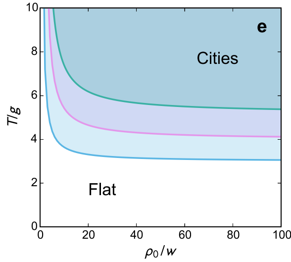
Fig. 60. Simulation result obtained in [187]. Cities emerge if the population is sufficiently mobile, i.e. if the migration rate T is sufficiently higher than the population growth rate g . The three curves show the conditions for the equilibrium state of uniform population to be unstable for the exponential IO model, Gravity models, and a power-law IO model (from bottom to top). Source: From [187].
