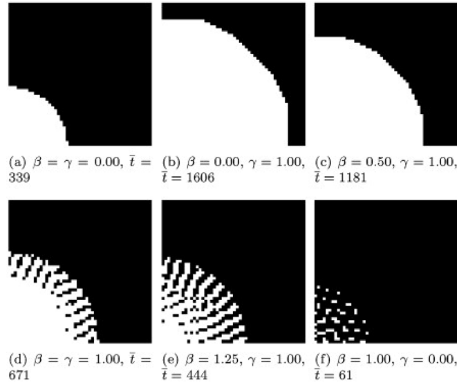
Fig. 31. Emergent urban forms in the Caruso et al. model. Simulated residential-agricultural patterns at the urban fringe, under varying strengths of green and social amenity preferences. Fragmented or compact morphologies emerge depending on parameter values.
